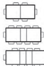
COL121 Extending Siena table H77xW190/230/270xD92 cm
